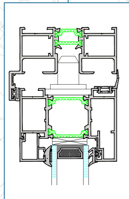
HEAD DETAIL
