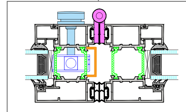
INTERMEDIATE DETAIL INTEGRATED LOCK
