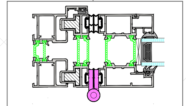
OUTER FRAME DETAIL WITH ADJUSTABLE JAMBS
